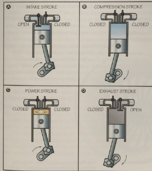
How a piston engine develops power
