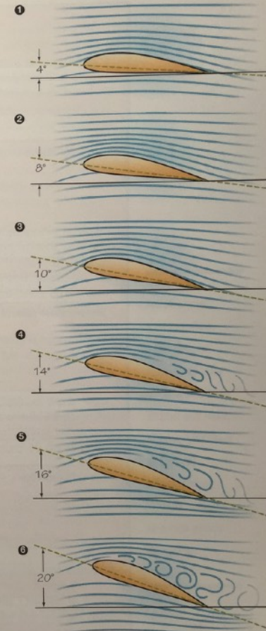
How airfoils work
